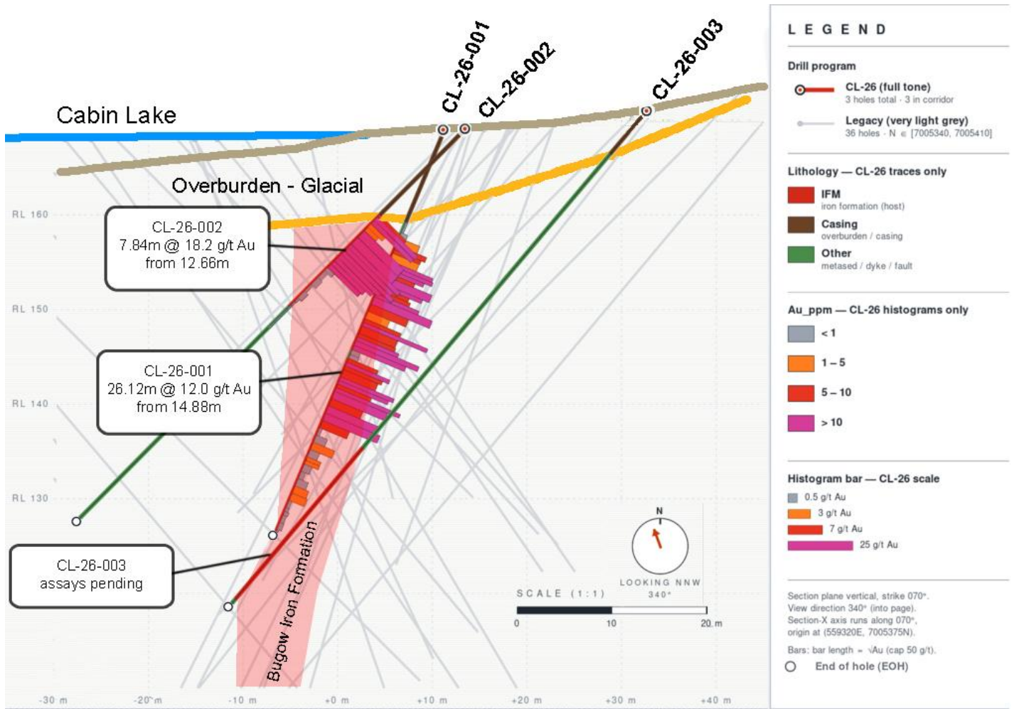
Figure 2. Section view of recently completed Arrow drillholes CL-26-001, CL-26-002 and CL-26-003.
